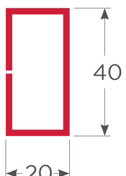
Ref. Inercia T 2mm - TC PL-CMP-TC-INT-2
