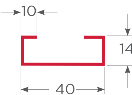
Ref. marco corredera 1.2mm - TC PL-SLD-TC-MCA-12
