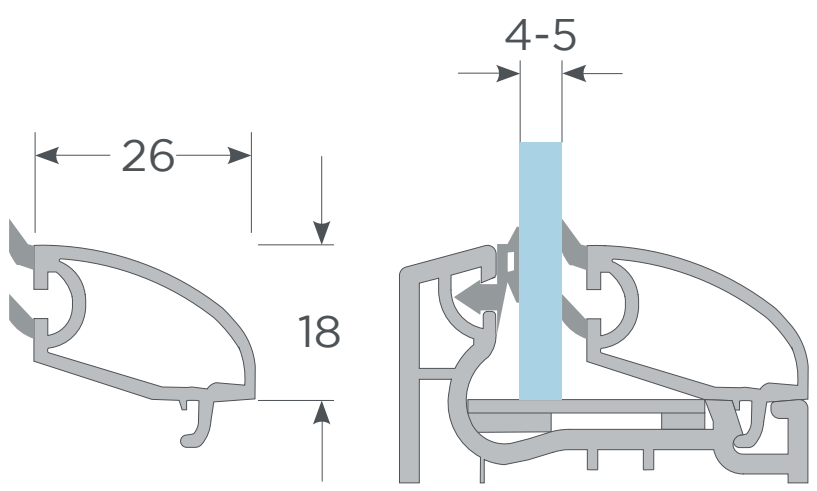
Junquillo 4-5mm Corredera
