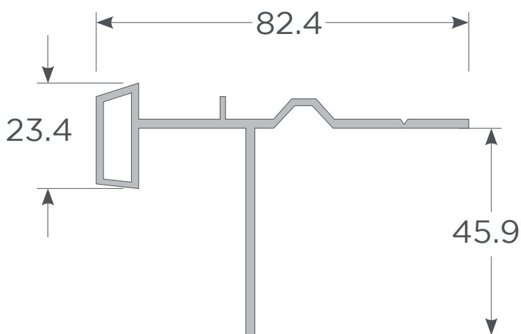
New Aleta Siding
