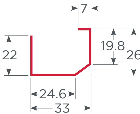
Ref. New Múltiple 1.2mm - TC PL-CMP-TC-MLT-12
