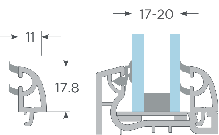
Junquillo 17-20mm Corredera
