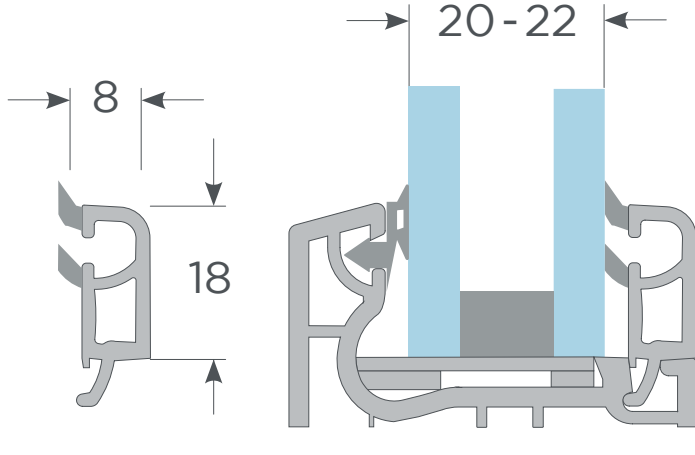
Junquillo 20-22mm Corredera
